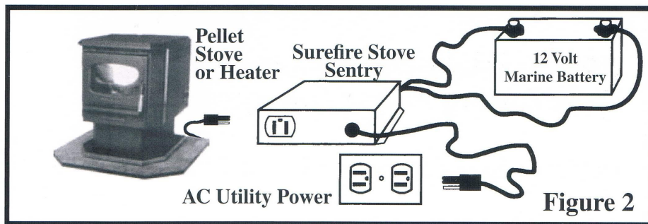
Figure 2 illustrates the interconnection between the pellet stove, Surefire Sentry and battery.
